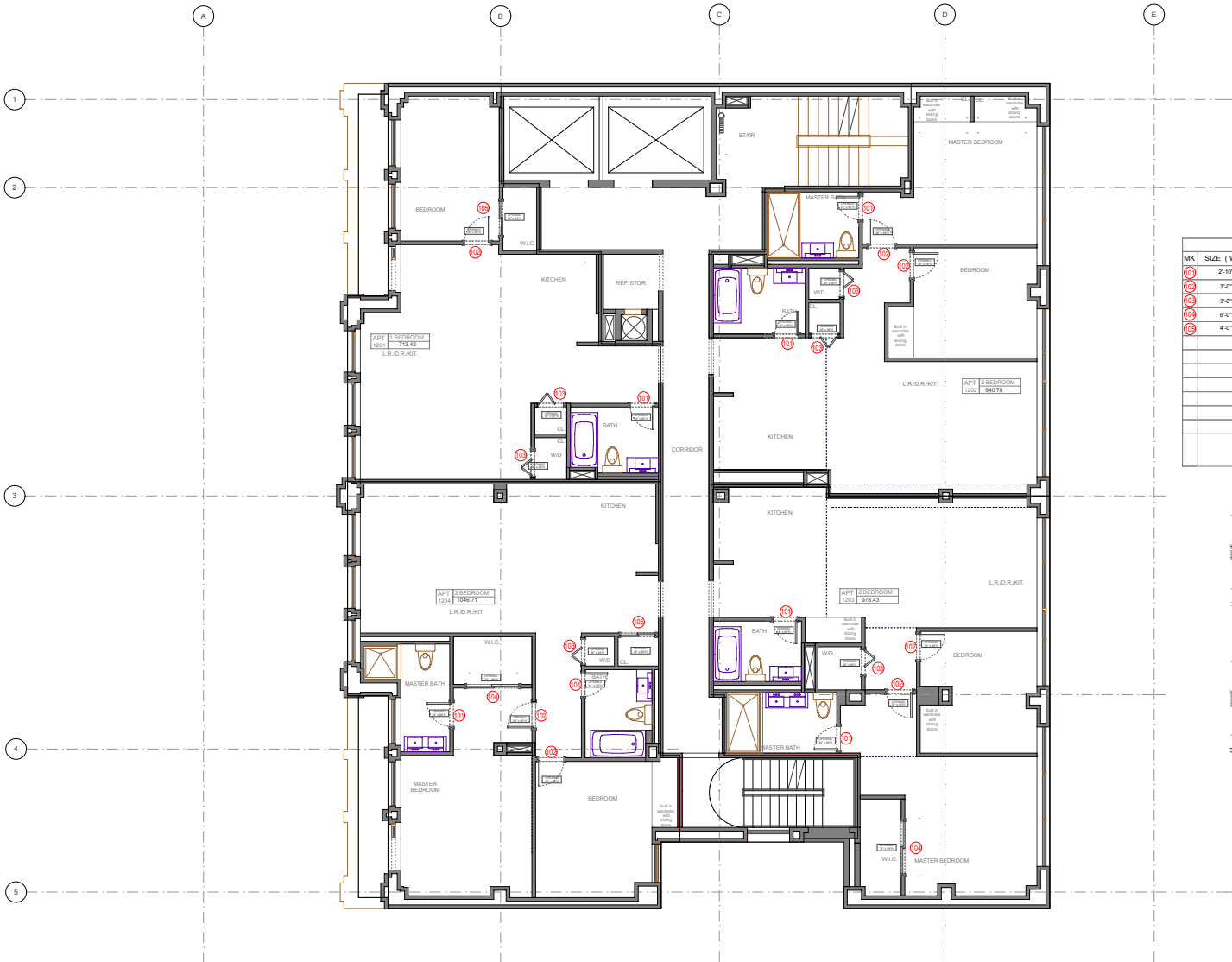
TWELFTH FLOOR PLAN GROSS AREA = 4543.13
